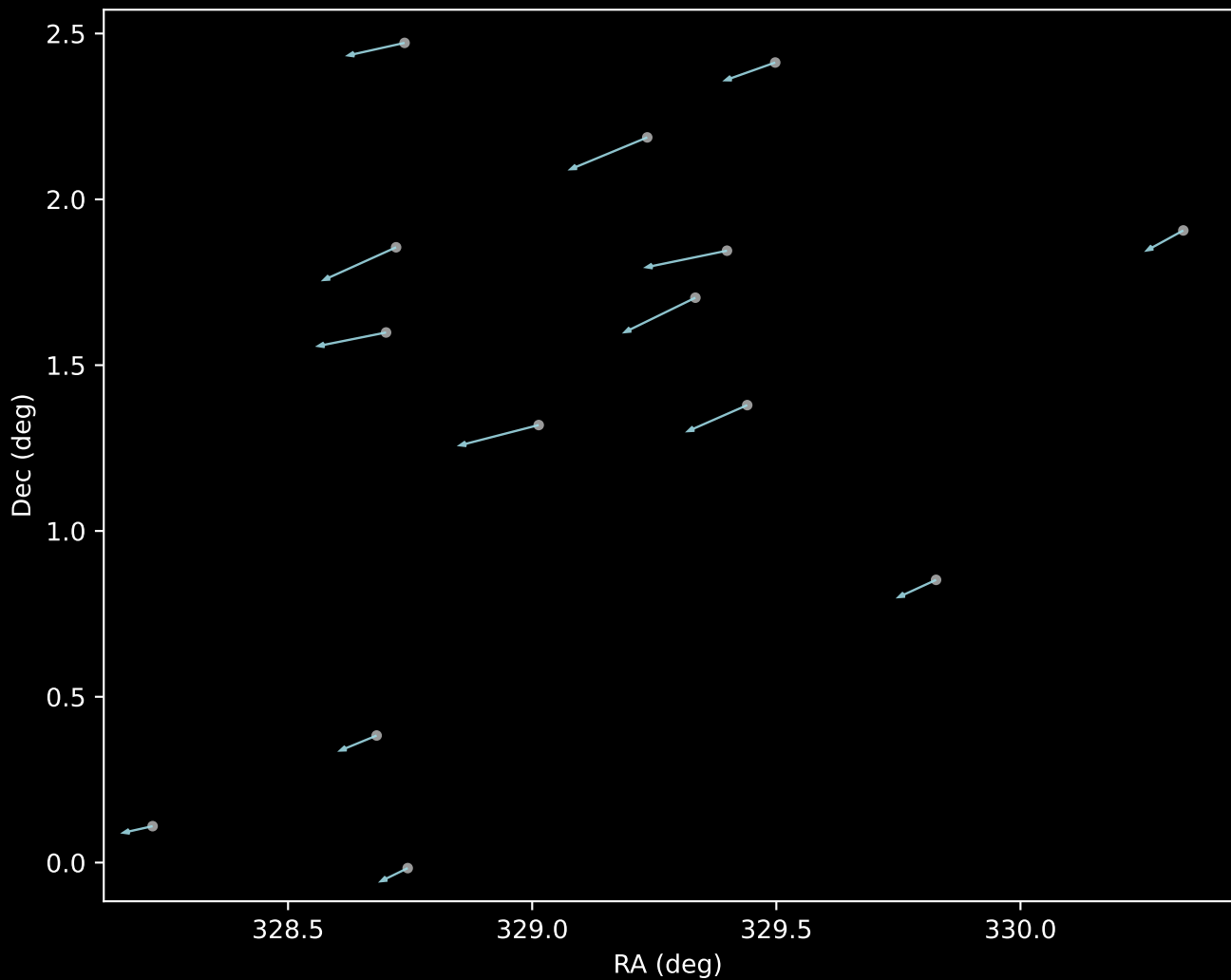
APOGEE DR17 Cluster 19 Proper Motion Vectors (n=14)
