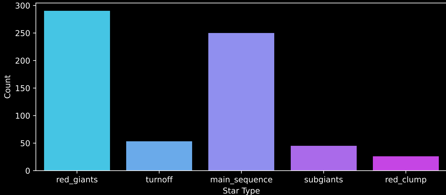
APOGEE DR17 Field: [M5PAL5] Count plot of Star Type
