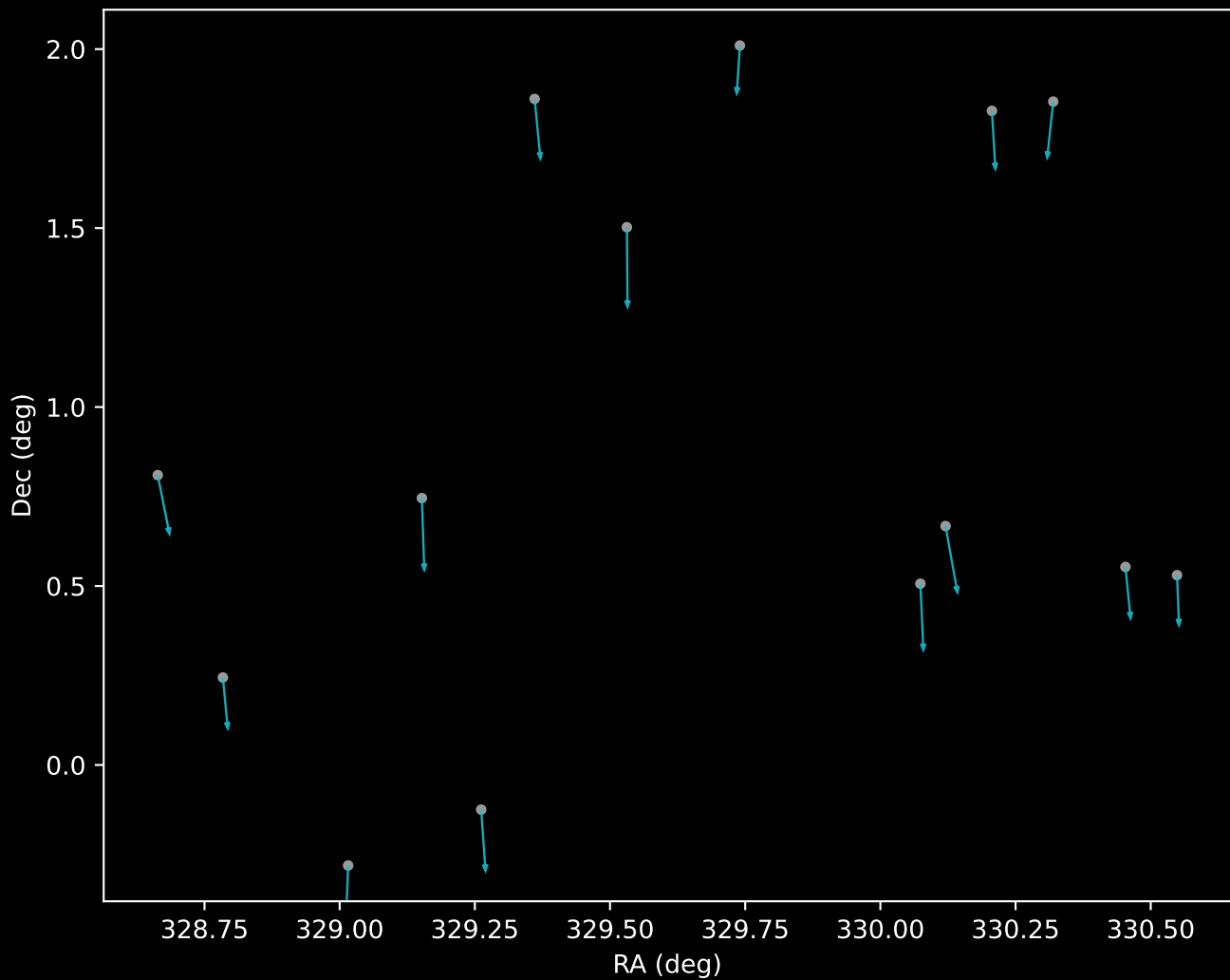
APOGEE DR17 Cluster 18 Proper Motion Vectors (n=14)
