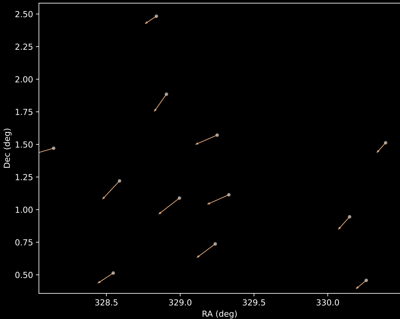
APOGEE DR17 Cluster 23 Proper Motion Vectors (n=12)
