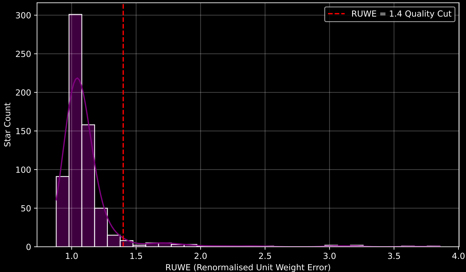
GAPOGEE DR17 Field [M5PAL5] RUWE Distribution (n= 653)
