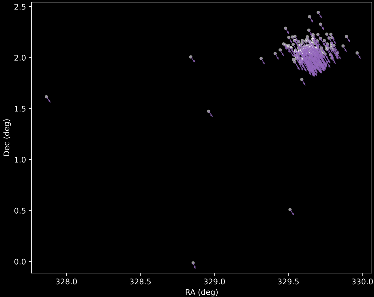
APOGEE DR17 Cluster 8 Proper Motion Vectors (n=158)
