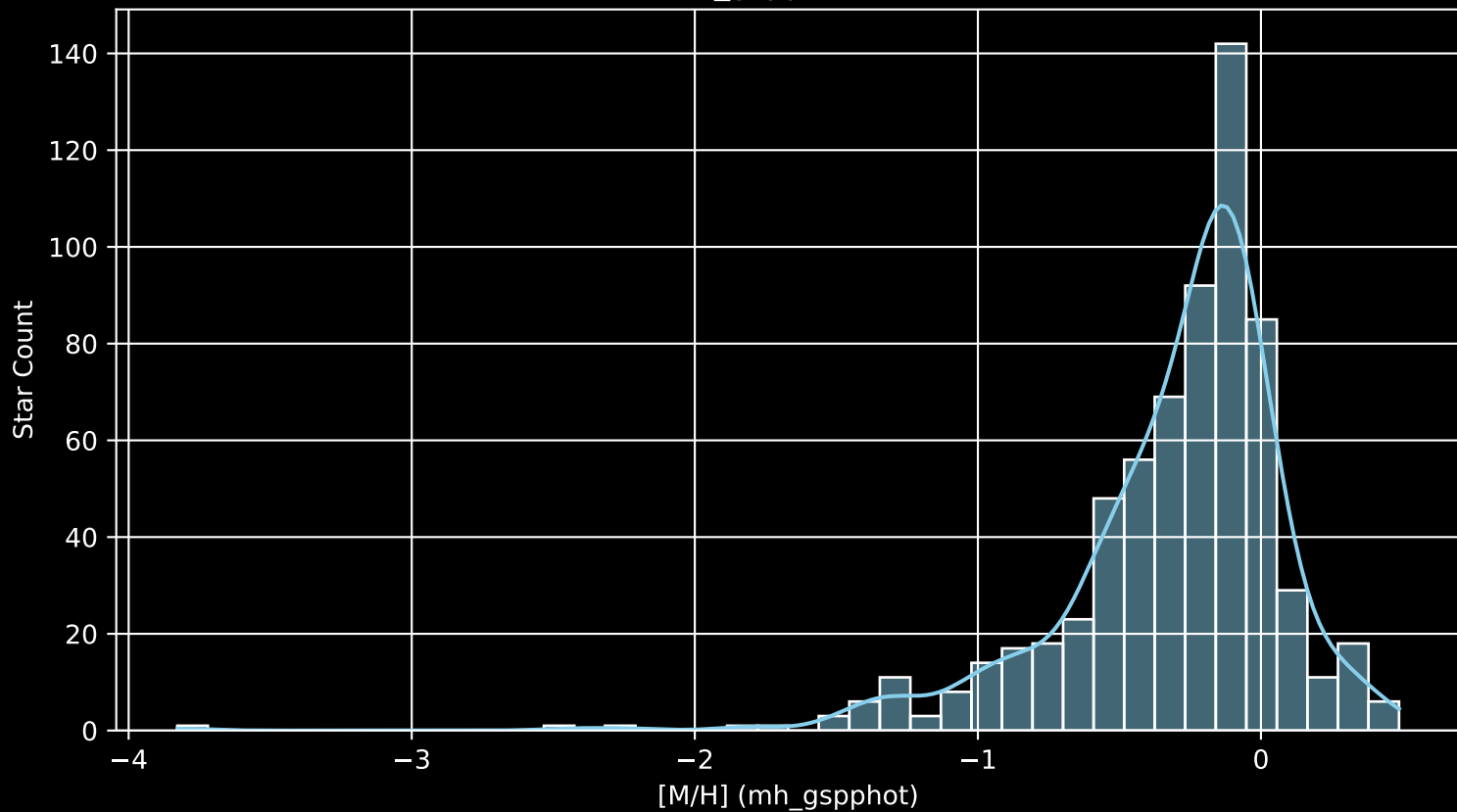
APOGEE DR17 Field: [M5PAL5 [M/H] (mh_gspphot) (n= 664)
