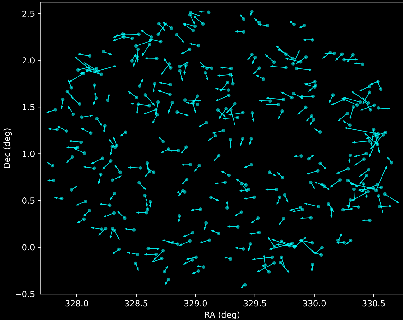
APOGEE DR17 Noise Stream Proper Motion Vectors (n=305)
