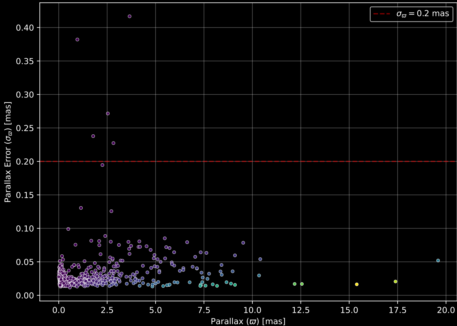
APOGEE DR17 Field: [M5PAL5] Parallax Quality (n= 664)
