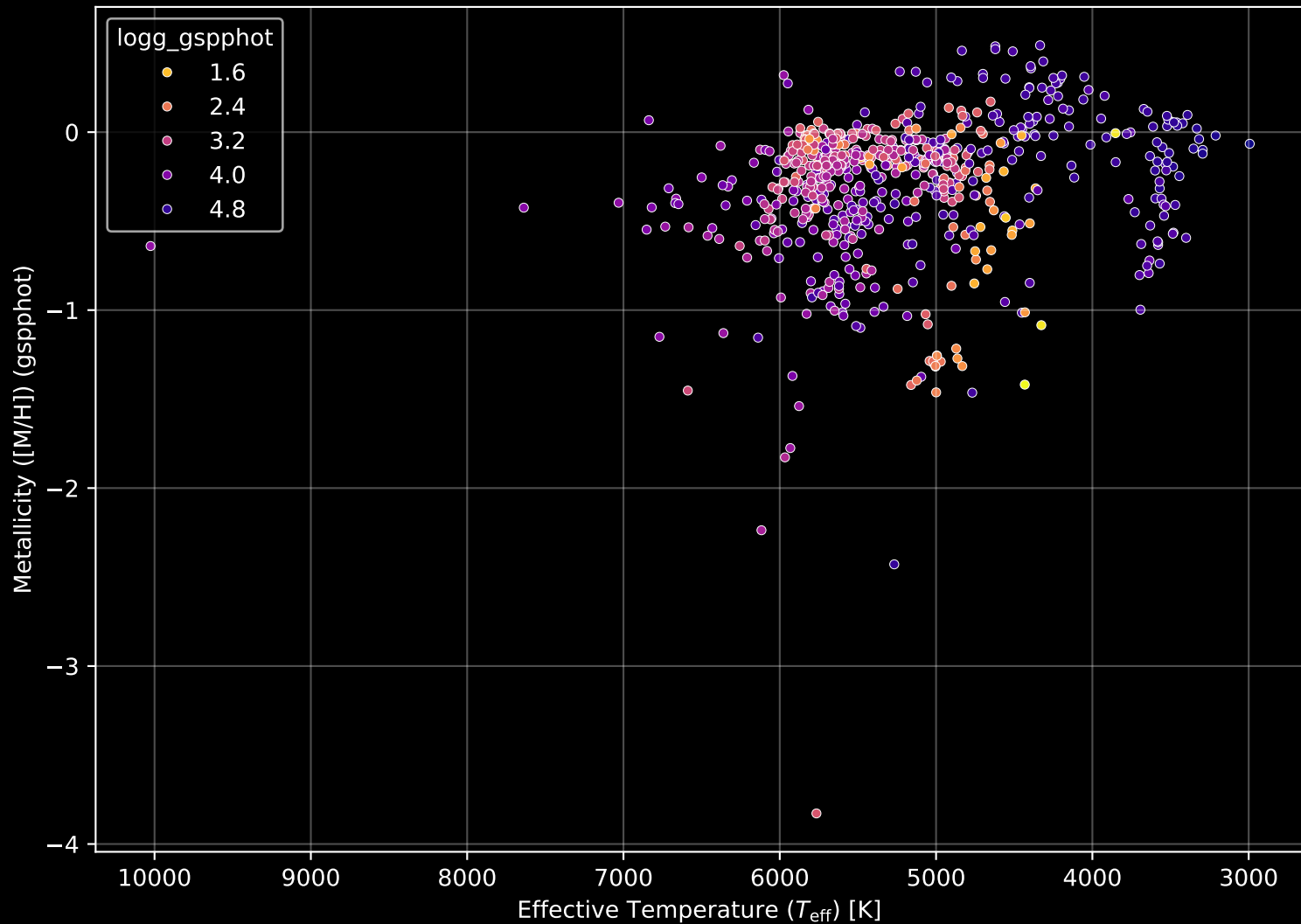
APOGEE DR17 Field: [M5PAL5] Stellar Population Parameters (n= 664)
