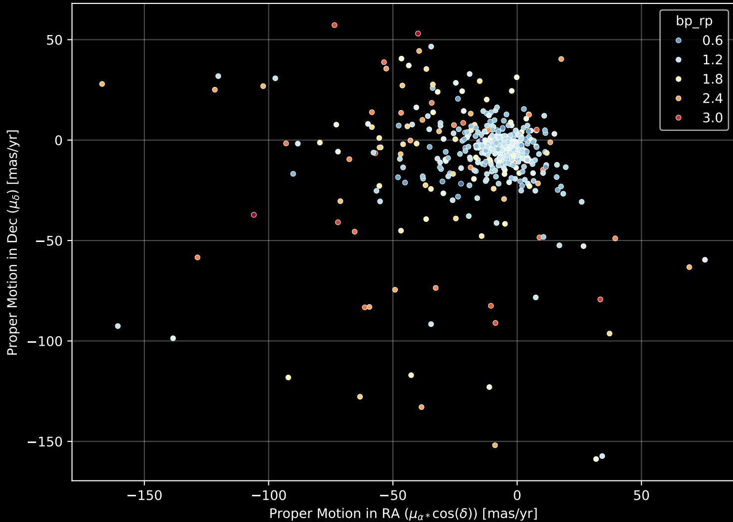
APOGEE DR17 Field: [M5PAL5] Proper Motion Diagram (n= 664)
